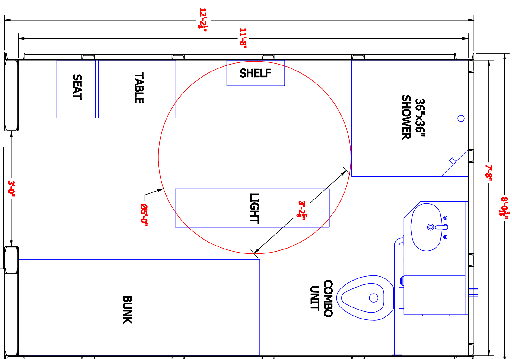
TYPE "2H1" REAR CHASE H.C. CELL ENGINEERED AREA: 35.8 SQ. FT. UNENGINEERED AREA: 54.7 SQ. FT. TOTAL AREA: 90.5 SQ. FT.
