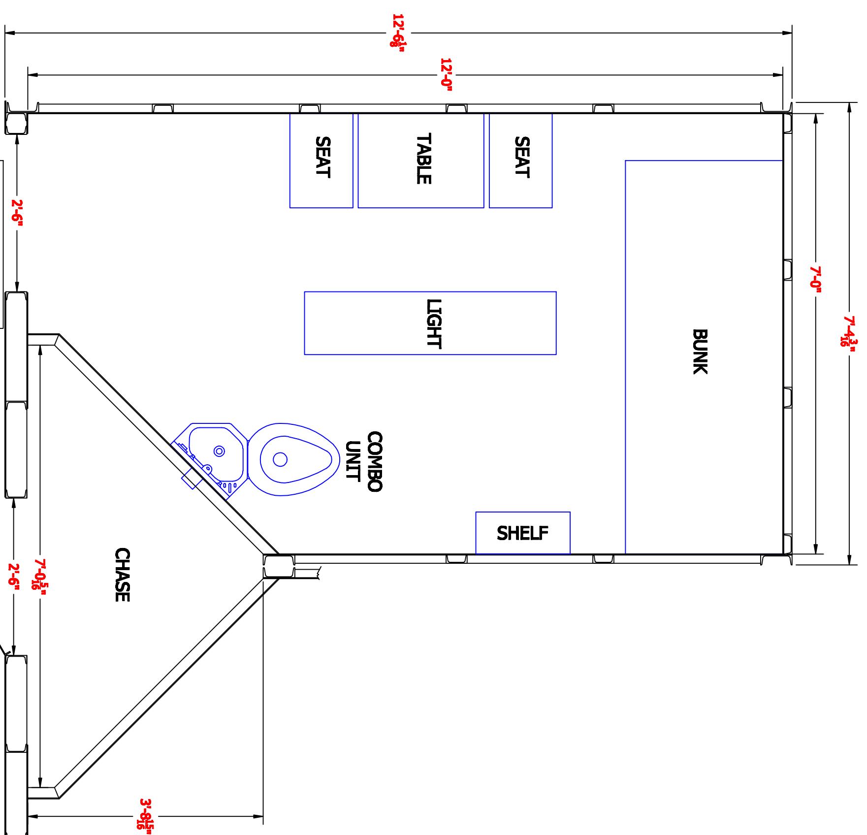
TYPE "1H3" FRONT CHASE CELL ENGINEERED AREA: 24.8 SQ. FT. UNENGINEERED AREA: 52.2 SQ. FT. TOTAL AREA: 77.0 SQ. FT.
