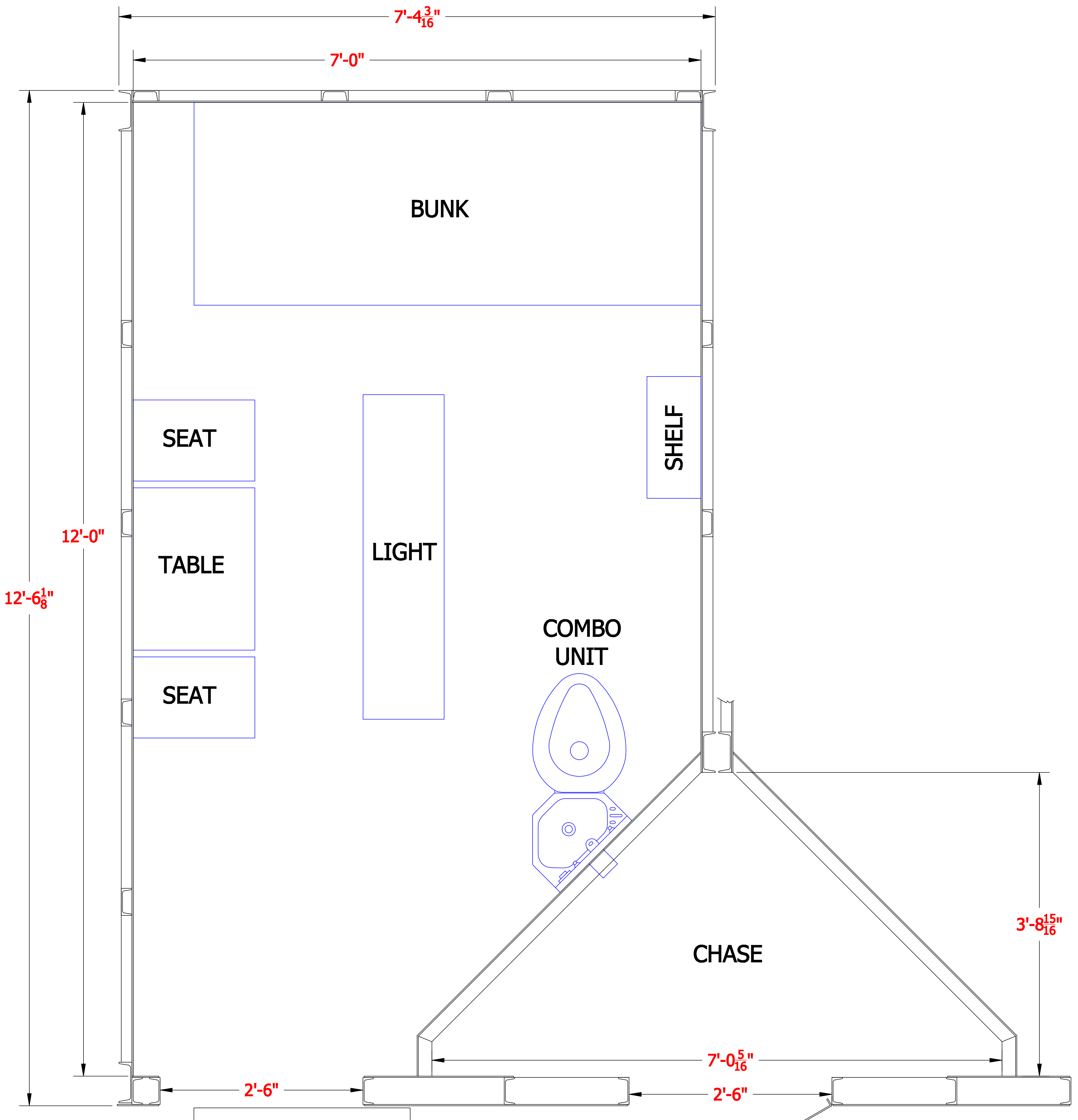
TYPE "3" FRONT CHASE CELL ENCUMBERED AREA: 24.8 SQ. FT. UNENCUMBERED AREA: 52.2 SQ. FT. TOTAL AREA: 77.0 Sq. Ft.
